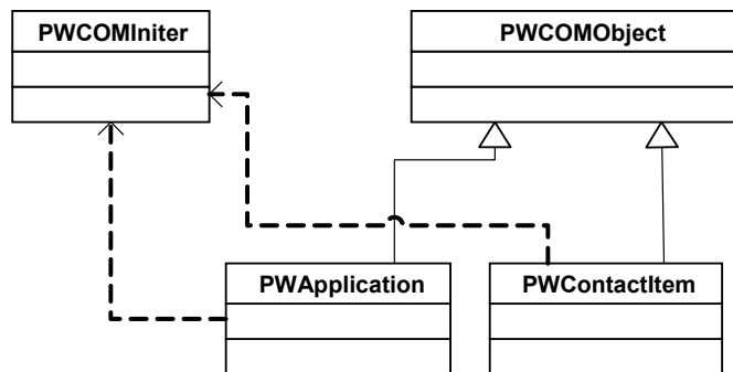
FIGURE 1.2 The relationship between the PWCOMObject and two of the Outlook COM objects, PWApplication and PWContactItem. The dotted arrows indicate that the child objects are reliant on a PWCOMIniter being instantiated for the current thread.
